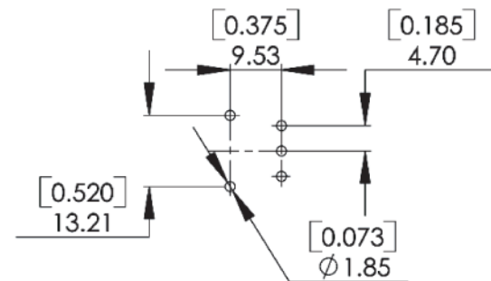
P.C. MOUNTING
