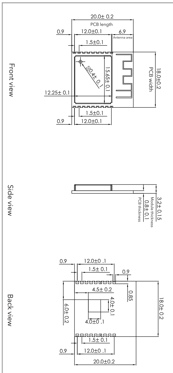
Figure 7-1. ESP-WROOM-02D Dimensions
