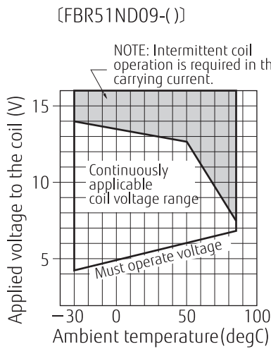
Operating Coil Voltage Range
