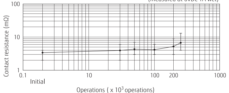
Contact resistance
