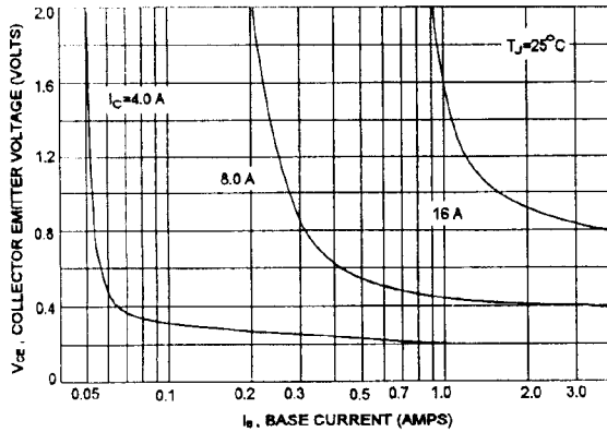
"ON" VOLTAGES
