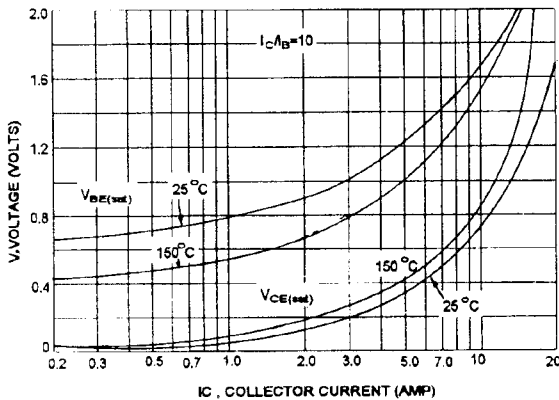
"ON" VOLTAGES
