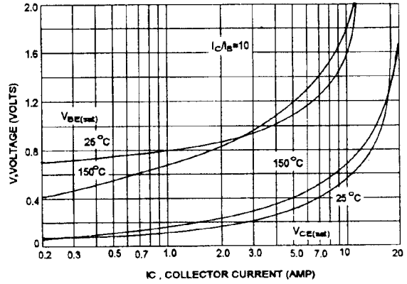
"ON" VOLTAGES
