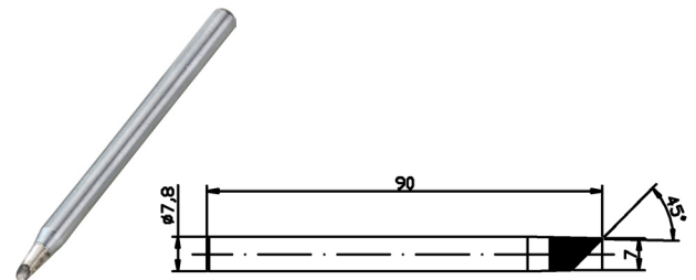
MP740171 Conical
