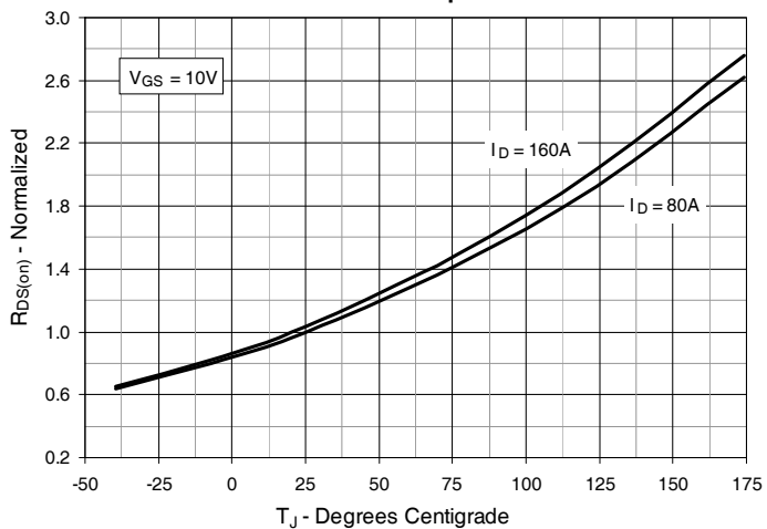
Fig. 4. R_{DS(on)} Normalized to I_D = 160A Value vs. Junction Temperature
